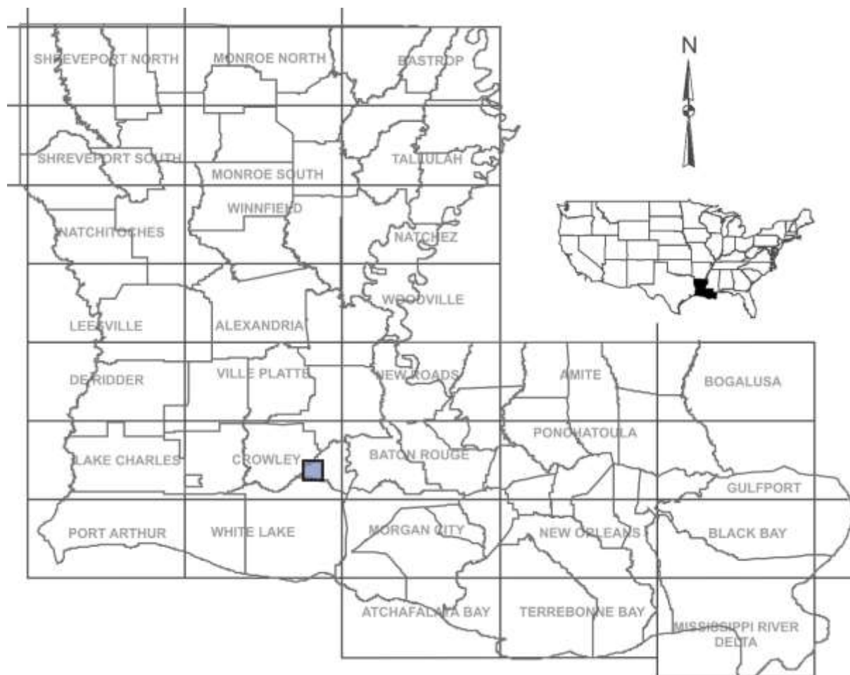
1. Location of Duson 7.5-minute quadrangle, southwestern Louisiana.
